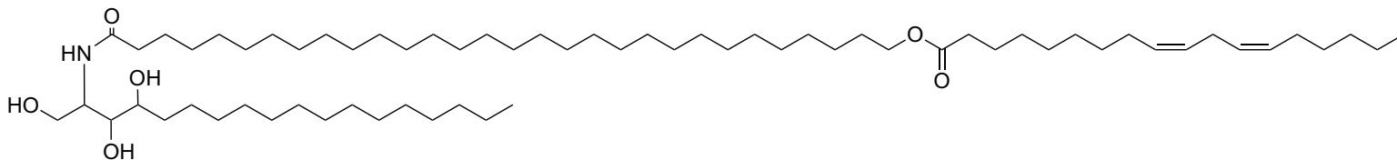
N-(30-Linoleoyloxy-triacontanoyl)-phytosphingosine
